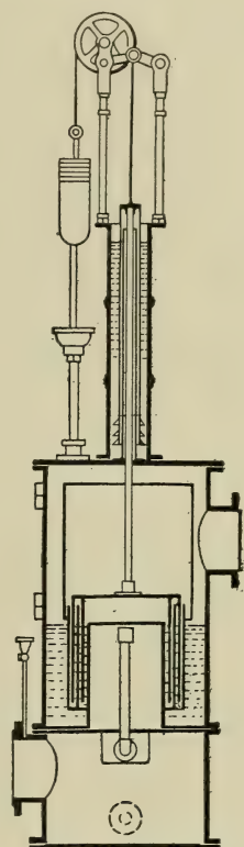
FIG. 69.—P. & A. Tar Extractor.
